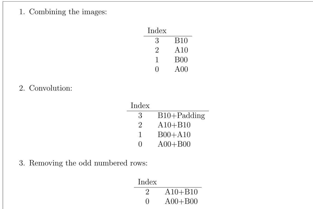
Figure 5: Example: Adding two 1×2 images, A and B.
